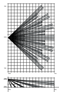
XCELW coverage
