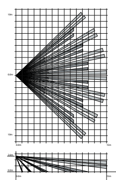
XCELR coverage
