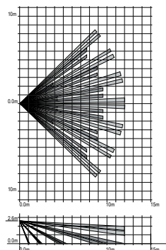
XCELWPT coverage
