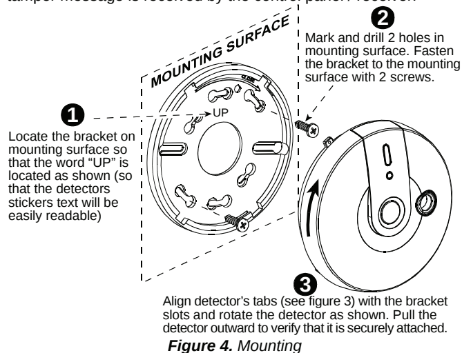
Figure 4. Mounting
