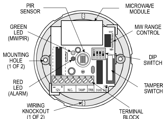
Figure 3. Component Layout
