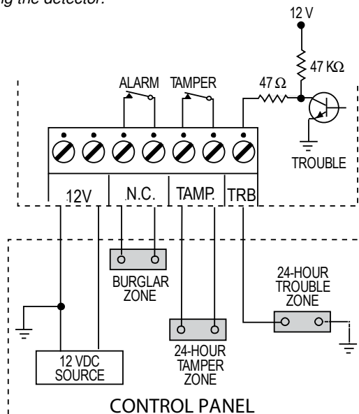
Figure 4. Terminal Block Wiring
