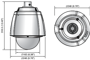
SCP-3370TH/3370H
